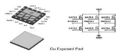
6 in 1 : 6*6*0.6
