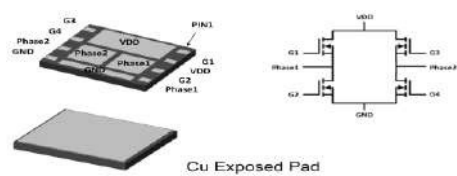
F-bridge : 5*6*0.6
