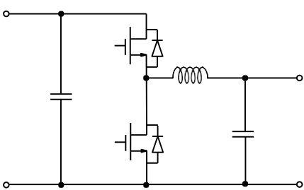
Synchronous Buck
